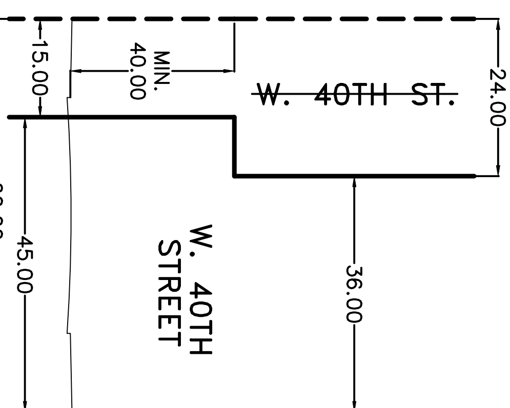
SECTION M-M TYPICAL CROSS SECTION OF VOLUME TO BE DEMAPPED OF WEST 40TH STREET N.T.S.
