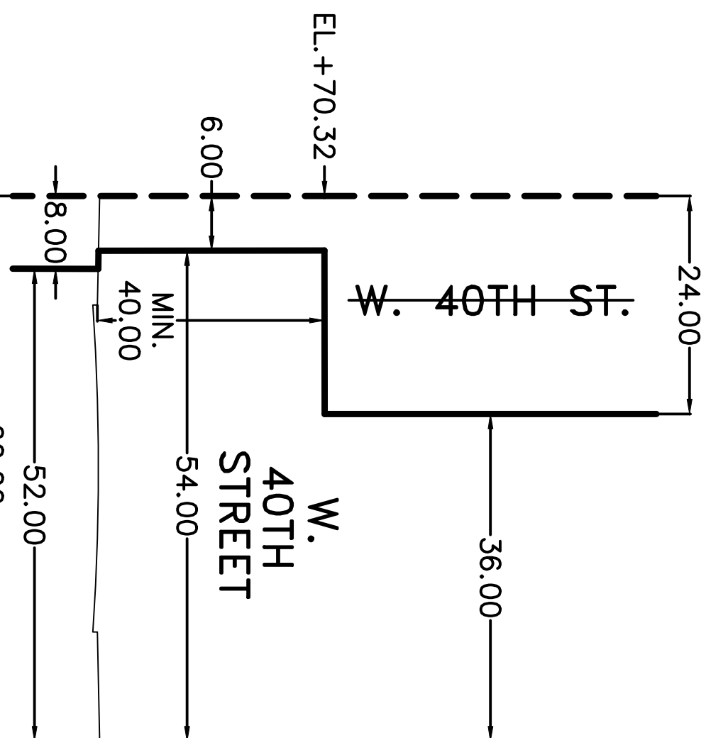
SECTION K-K TYPICAL CROSS SECTION OF VOLUME TO BE DEMAPPED OF WEST 40TH STREET N.T.S.
