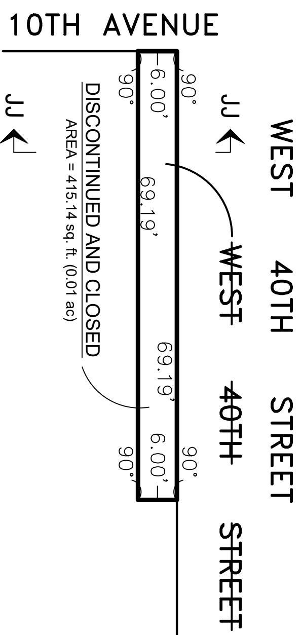
DISCONTINUANCE AND CLOSING DETAIL 5
