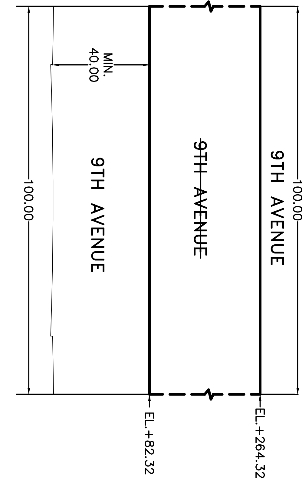
SECTION F-F TYPICAL CROSS SECTION OF AERIAL VOLUME TO BE DEMAPPED ABOVE 9TH AVENUE N.T.S.
