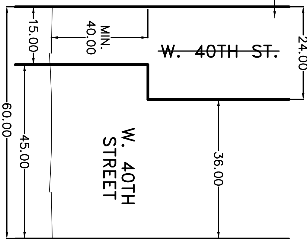
SECTION LL-LL TYPICAL CROSS SECTION OF VOLUME TO BE DEMAPPED OF WEST 40TH STREET N.T.S.
