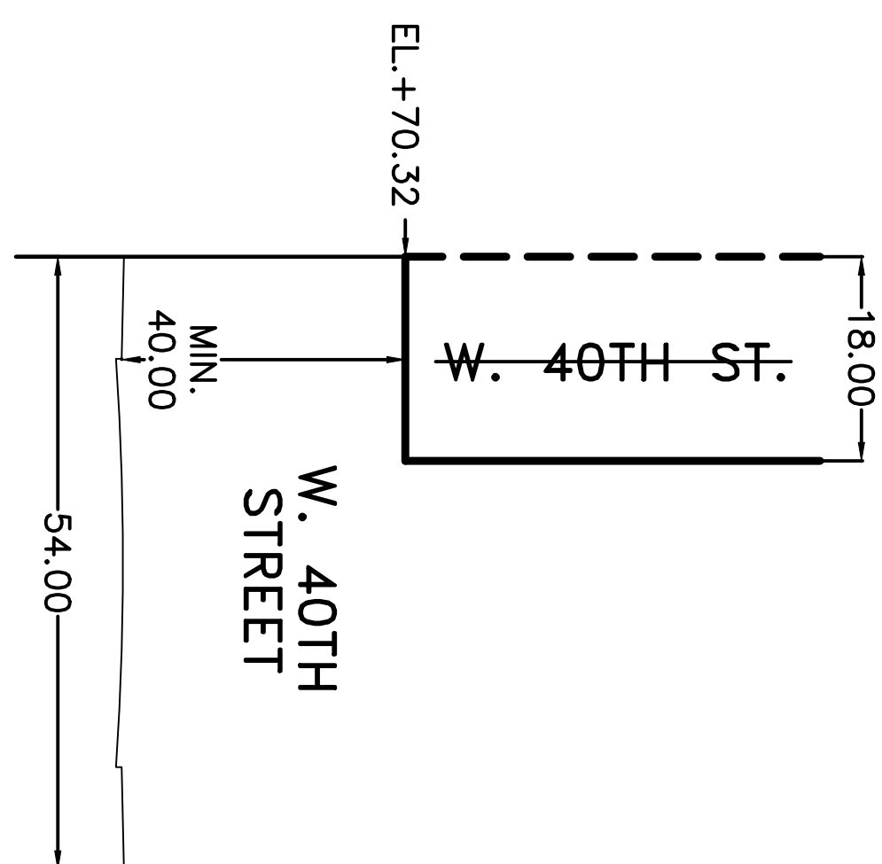
SECTION J-J TYPICAL CROSS SECTION OF AERIAL VOLUME TO BE DEMAPPED ABOVE WEST 40TH STREET N.T.S.
