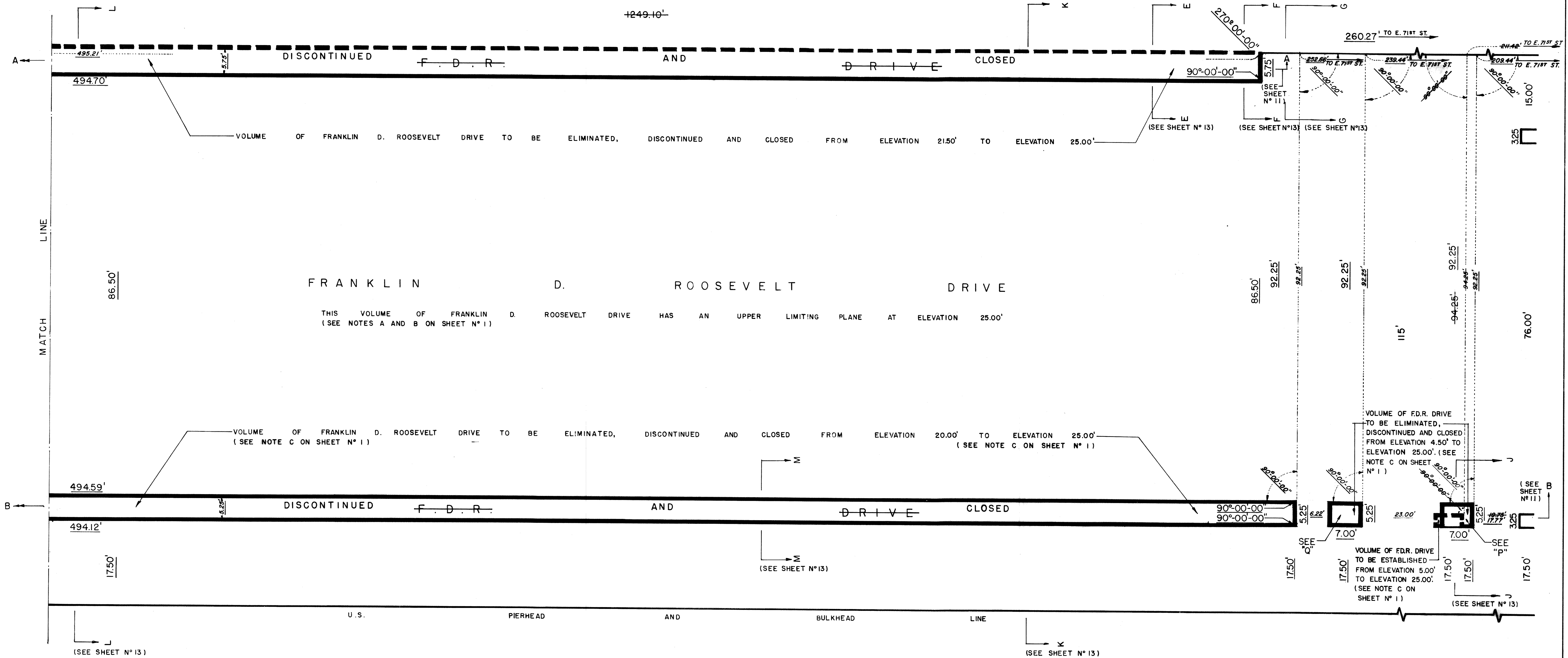
PLAN AT ELEVATION 23.00' SHOWING VOLUMES OF FRANKLIN D. ROOSEVELT DRIVE TO BE ELIMINATED, DISCONTINUED AND CLOSED. SCALE : 1" = 10'
