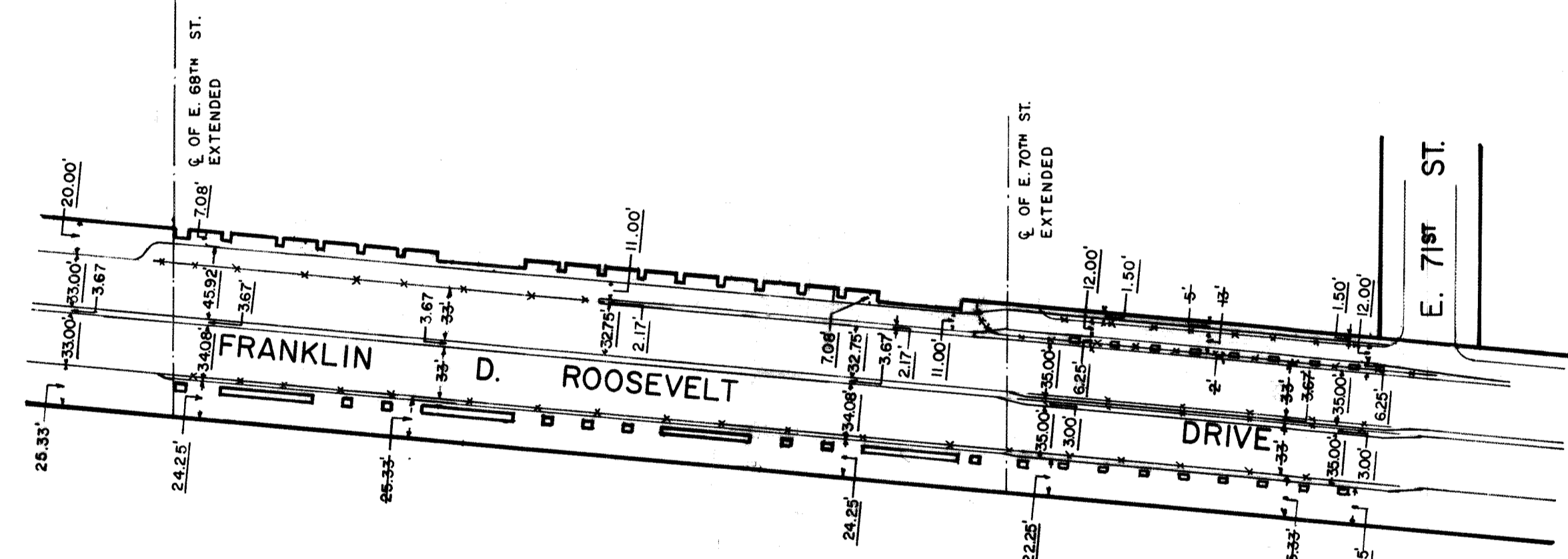
AT-GRADE PLAN SHOWING MODIFICATION TO STREET TREATMENT SCALE 1" = 80'
