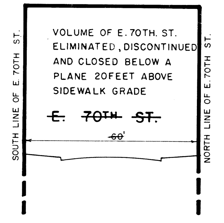
SECTION A - A SCALE HOR. - 1" = 20'
