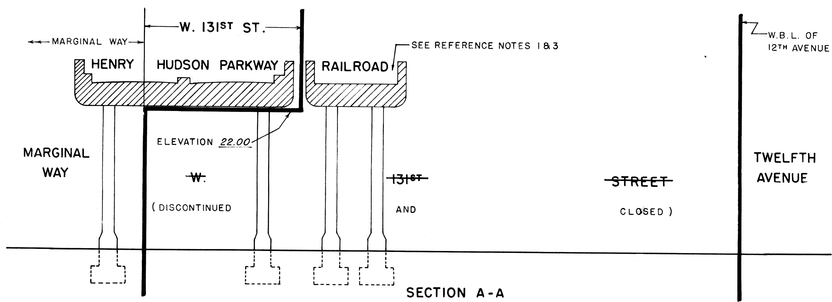
SECTION A-A SCALES HOR. 1" = 20" VERT. NOT TO SCALE
