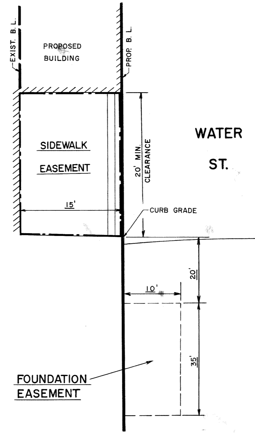
SECTION A-A TYPICAL SIDEWALK ARCADE (NOT TO SCALE)
