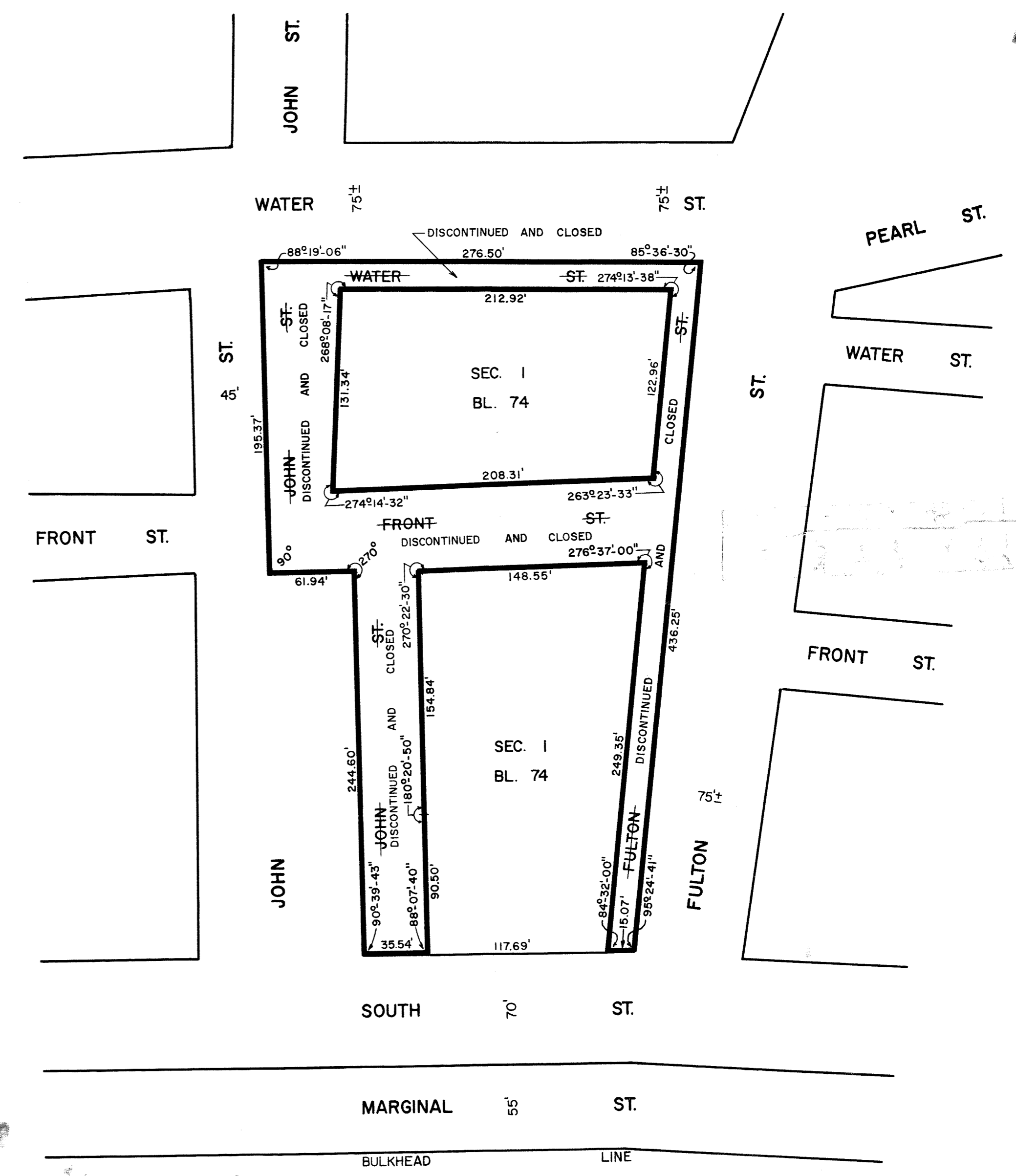
PLAN SCALE: 1"=60'
