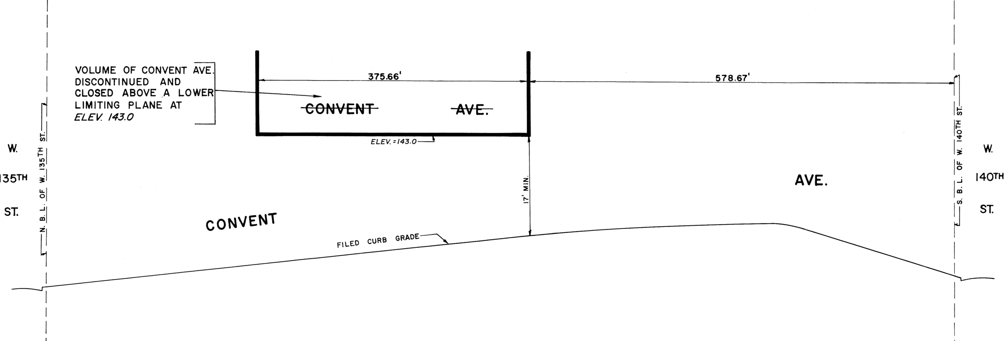
SECTION A-A SCALE: HOR: 1" = 80' VERT: 1" = 10'
