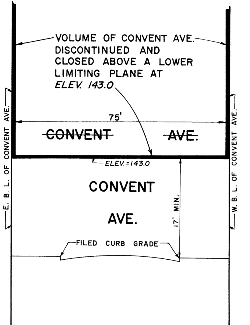
SECTION B-B SCALE: HOR: 1" = 20' VERT: 1" = 10'
