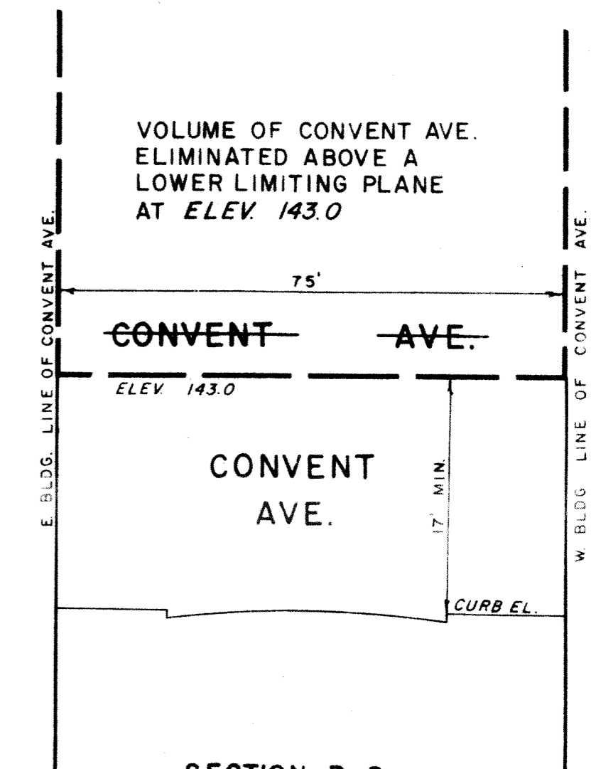
SECTION B-B HOR. 1"=20' VERT. 1"=10'
