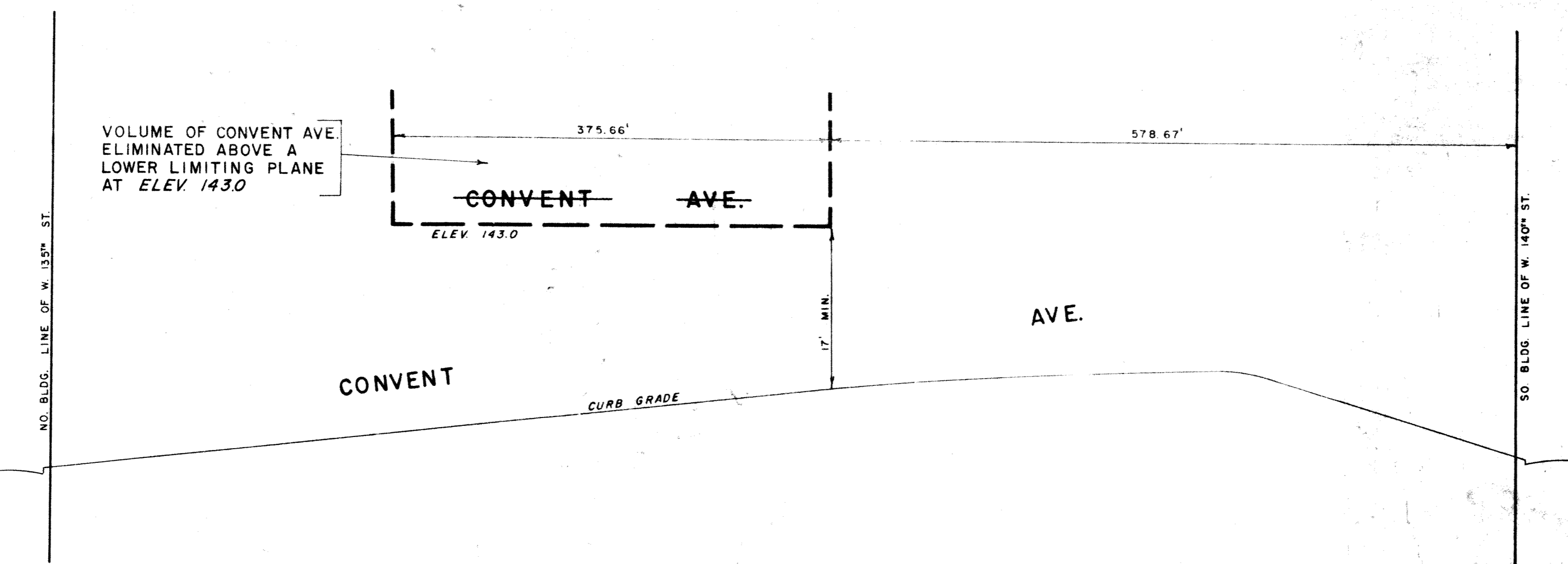
SECTION A-A HOR. 1"=80' VERT. 1"=10'
