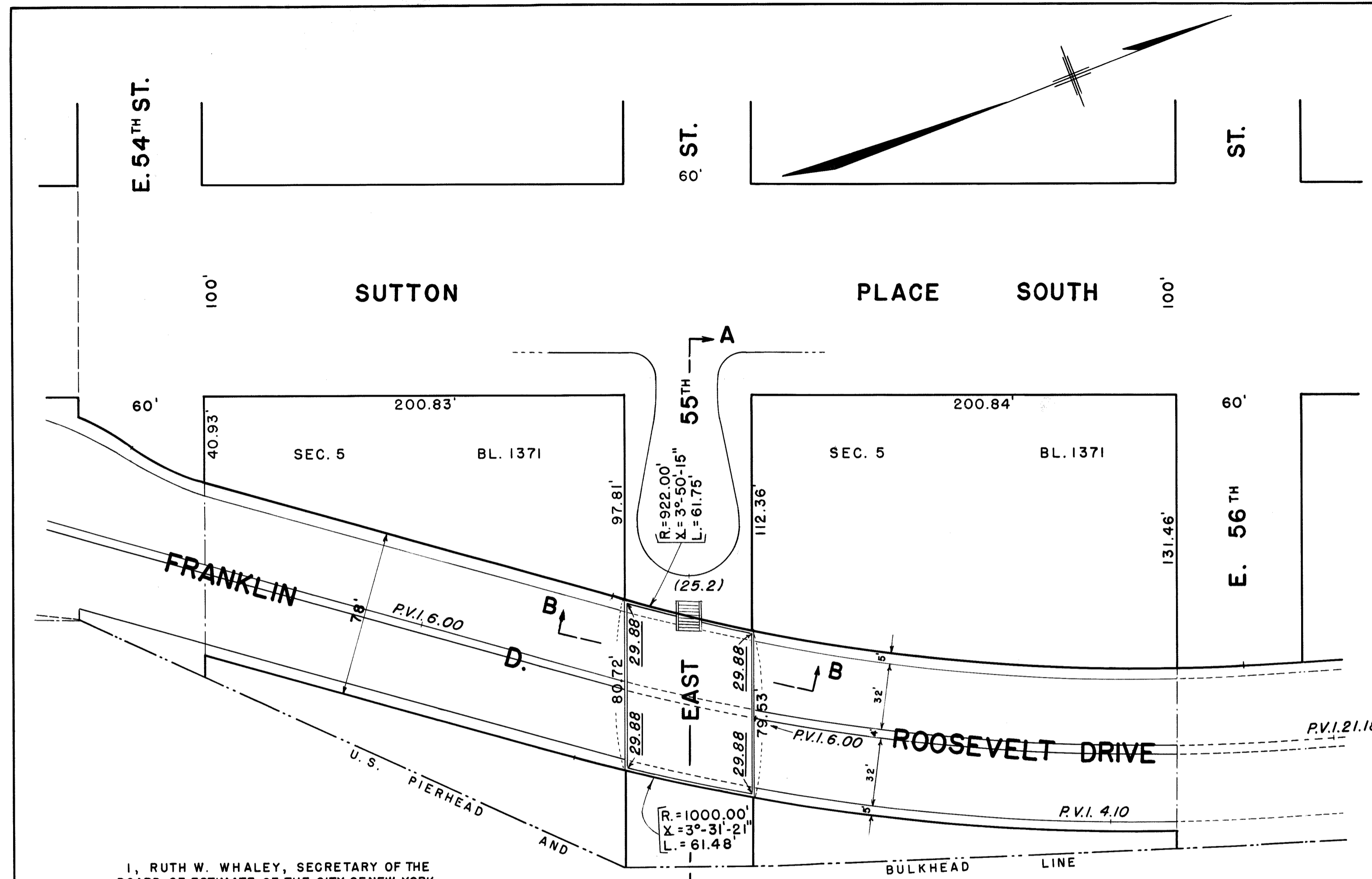
PLAN SCALE 1" = 40'
