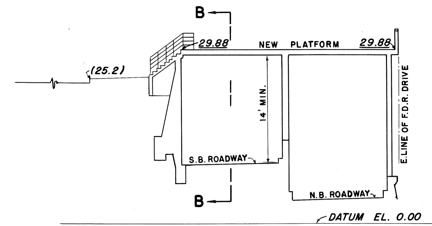
SECTION A-A SCALES: HORIZ. 1" = 20', VERT. 1" = 10'
