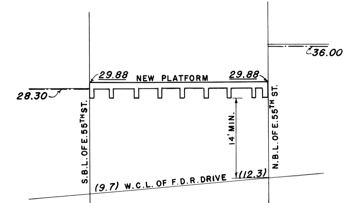
SECTION B-B SCALES: HORIZ. 1" = 20', VERT. 1" = 10'
